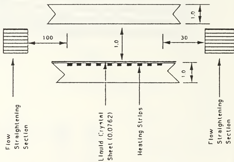
Figure 4. Side view of test surface. Dimensions in cm.
